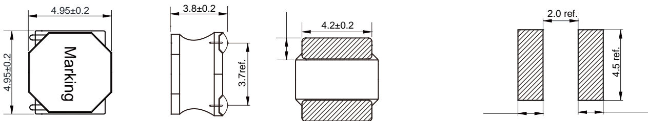
Land Pattern: [mm]
