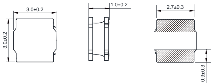
Dimensions: [mm]
